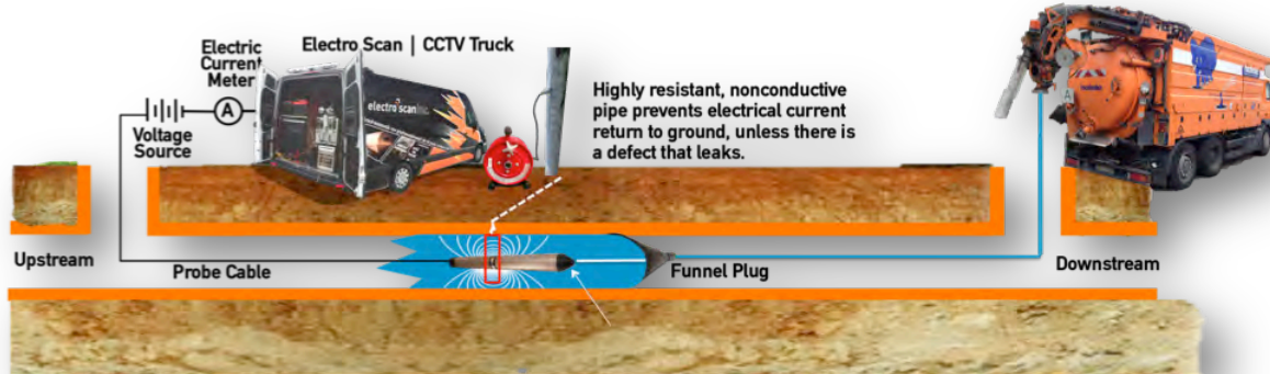
Figure 12 - Electric Circuitry of a Sewer System,
