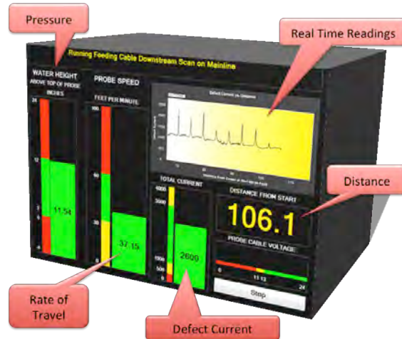
Figure 16. Data automatically displayed on Operator's Real Time Console, requiring no data entry or interpretation during scanning process.
