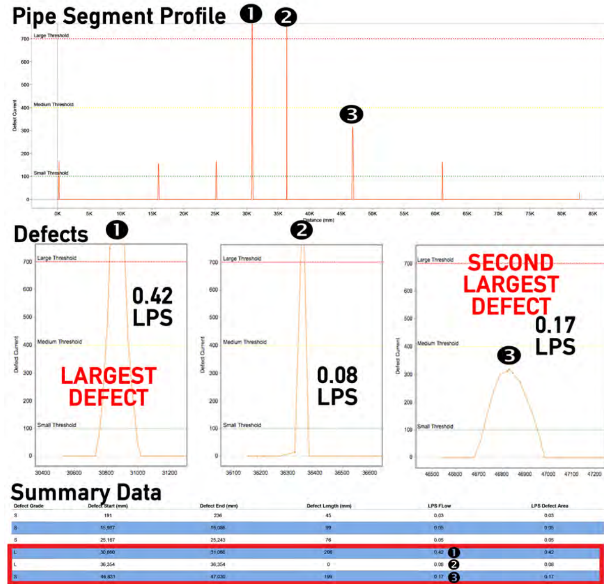
Figure 4. Individual scanned pipes, ranked sixth (6 th ) out of a total of 49 pipe segments. Total pipe segment defect flow of 19,066 GPD, .084 LPS, or 72,190 LPD), including two (2) Large Defects and five (5) Small Defects. 00000180_apr012014_145714PM
